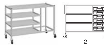
Name: Treble combination trolley Ref: 3020 1 Size: H725 x W1055 x D420mm 2 Size: H850 x W1055 x D420mm
