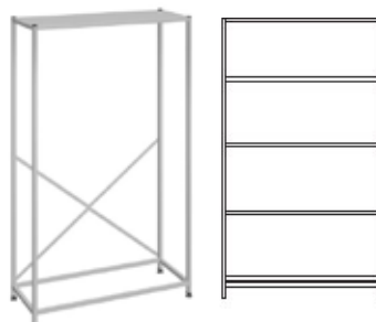
Name: Tall treble width frame Ref: 3622 Size: H1850 x W1055 x D420mm
