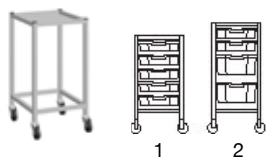
Name: Single column trolley Ref: 1025 1 Size: H725 x W370 x D420mm 2 Size: H850 x W370 x D420mm
