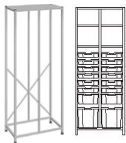
Name: Tall double column frame Ref: 2625 Size: H1850 x W710 x D420mm
