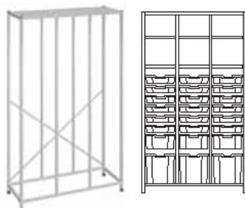
Name: Tall treble column frame Ref: 3625 Size: H1850 x W1055 x D420mm
