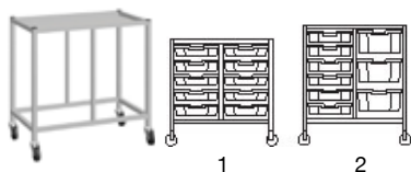
Name: Double column trolley Ref: 2025 1 Size: H725 x W710 x D420mm 2 Size: H850 x W710 x D420mm
