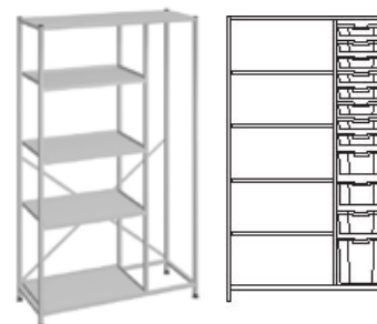
Name: Tall treble combination frame Ref: 3620 Size: H1850 x W1055 x D420mm
