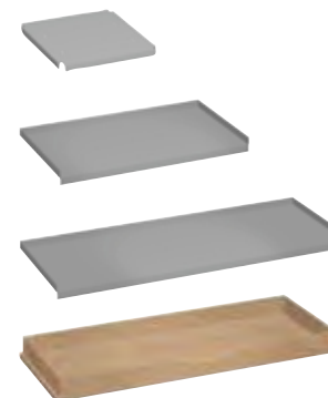
Name: Treble width shelf Ref: 363 Size: H40 x W1055 x D420mm
